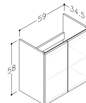
MDO636WH Metro wall hung vanity unit -600mm- 2 Door with basin Short projection -360MM Colour - Glossy White £435.00
