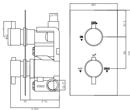
CR1220 Cross 2 handle thermostatic concealed shower valve 1 outlet £279.00
