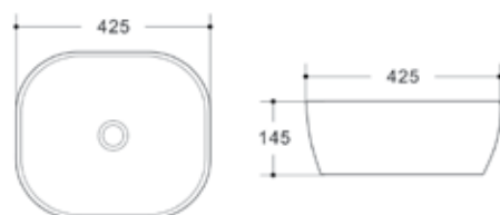
AB425G Art Basin-Counter top Size 425*425*145MM Colour -Gold £669.00
