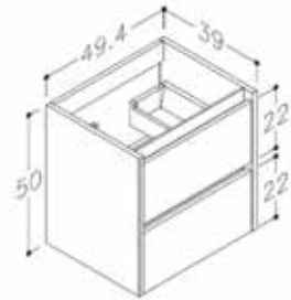
CW539WH City wall hung vanity unit -500mm Colour - Glossy White £415.00
