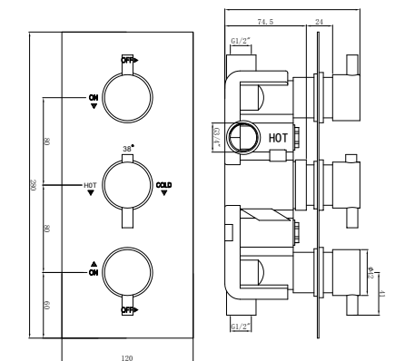
MS1430CH Square 3 handle thermostatic concealed shower valve 2 outlets £389.00
