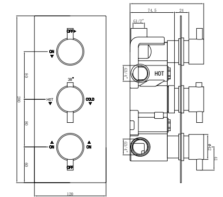
MS1435CH Square 3 handle thermostatic concealed shower valve 3 outlets £395.00
