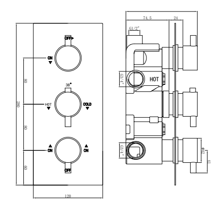
CR1235 Cross 3 handle thermostatic concealed shower valve 3 outlets £389.00
