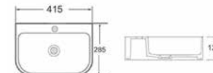
RCB703 Round ceramic basin Size: 415*285*125MM £115.00
