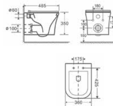
RO130SP Rio Wall Hung Short Projec- tion WC Pan with soft close seat £360.00
