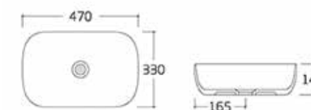
AB800 Counter top ceramic basin Size: 470*330*140MM £169.00
