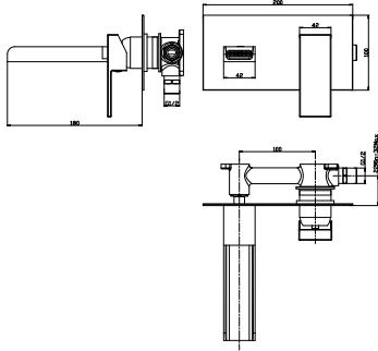
WF110P Waterfall wall mounted single lever basin mixer £175.00
