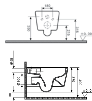
TRV130MB Treviso wall hung toilet with soft close seat Size: 490*370*370MM Colour- Matt Black £995.00
