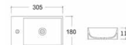
SSB704 Square ceramic basin Size: 305*180*110MM £95.00
