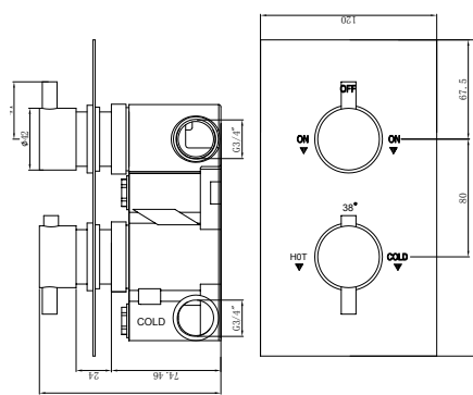
MS1425CH Square 2 handle thermostatic concealed shower valve 2 outlets £350.00
