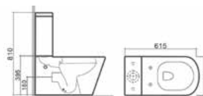
RC110 Richmond close coupled WC pan with soft close UF seat cover £447.00
