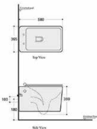
RO580 Rio Wall Hung Toilet £330.00
