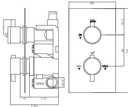
MS1420CH Square 2 handle thermostatic concealed shower valve 1 outlet £299.00
