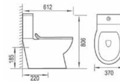
BE150 Bergen close coupled WC pan with soft close UF seat cover £375.00
