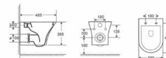
ED130 Eden wall hung WC pan with soft close UF seat cover £350.00
