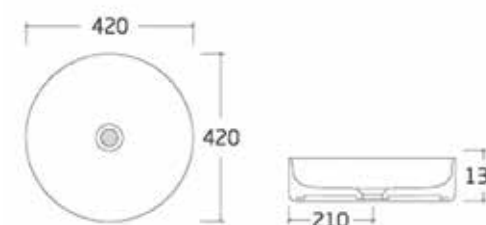
AB804 Counter top ceramic basin Size: 420*420*135MM £135.00
