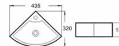
CAB701 Corner ceramic basin Size: 435*320*130MM £95.00
