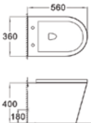
RG120 Riga back to wall WC pan with soft close UF seat cover £319.00
