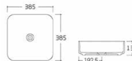
AB801 Counter top ceramic basin Size: 385*385*135MM £150.00
