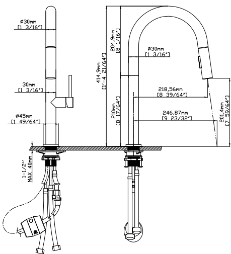
TRV150BGB Grace single lever kitchen mixer (Black) £325.00
