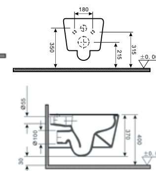
TRV130B Treviso wall hung toilet with soft close seat Size: 490*370*370MM Colour- Black £1199.00
